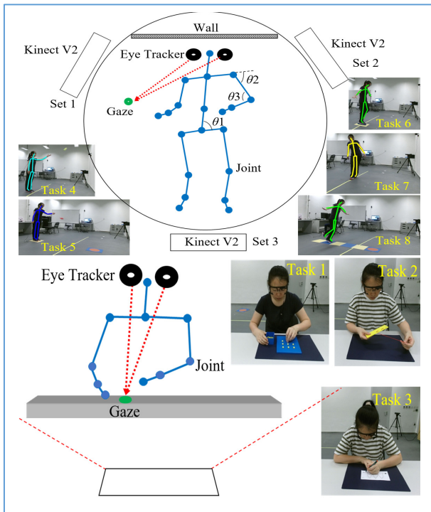
Figure 2 A marker-less digitalized system for DCD assessment
